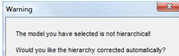
Hierarchy warning
